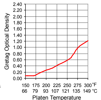
Static Sensitivity
